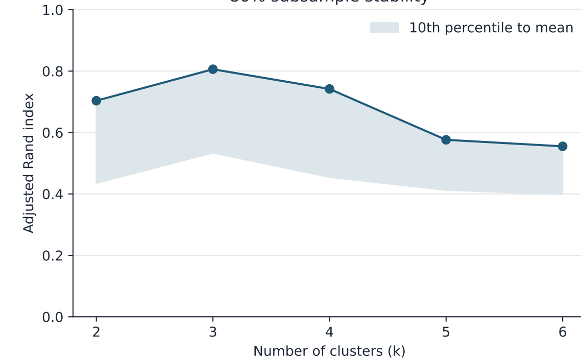
80% subsample stability
