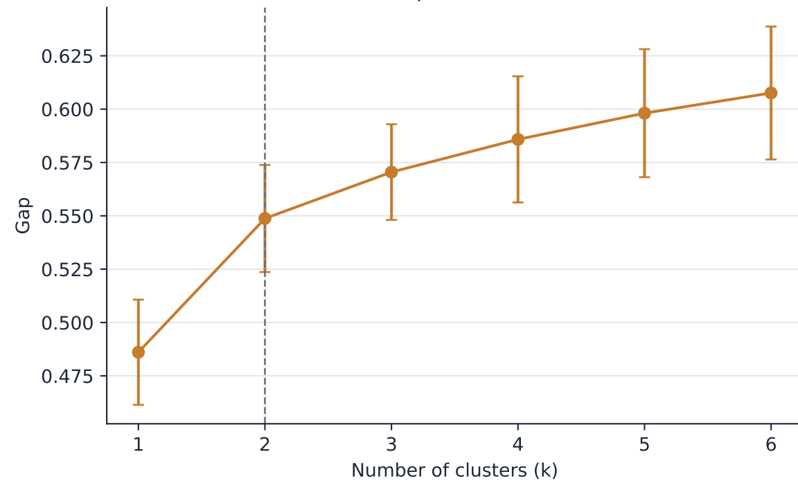
Gap statistic
